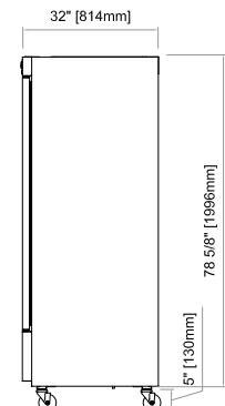
QVR(F) Common View
