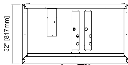
QVR(F)-2 Top View
