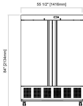
QVR(F)-2 Front View
