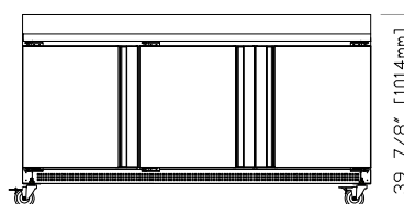
FWR-72 Front View
