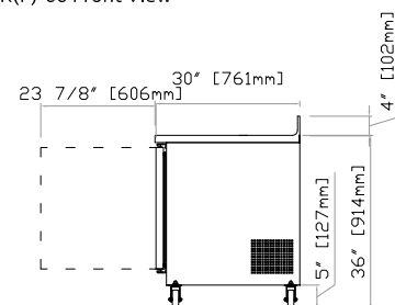
FWR(F)-60 Front View
