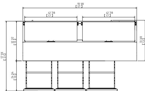
FPT-93-D6 Top View
