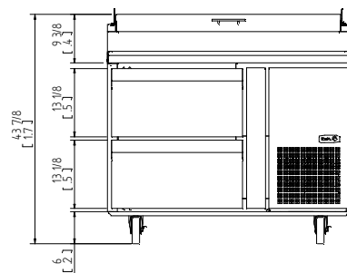
FPT-46-D2 Front View
