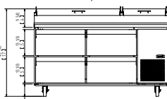
FPT-67-D4 Front View
