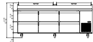
FPT-93-D6 Front View
