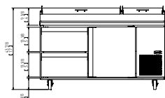
FPT-67-D2 Front View
