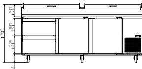
FPT-93-D2 Front View
