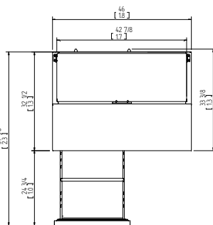
FPT-46-D2 Top View
