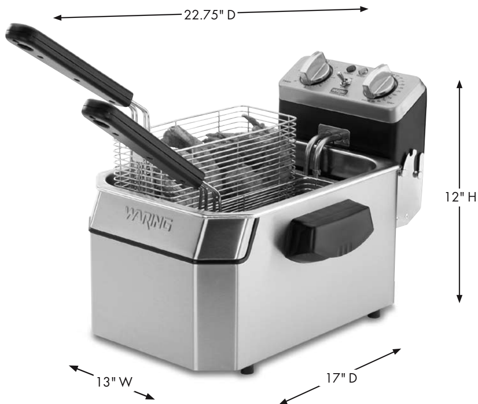
WDF1000/WDF1000B
