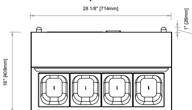
CPR-60-4 Top View
