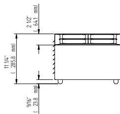
CPR-8 Front View
