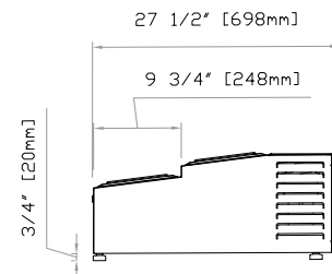
CPR-60-4 Side View
