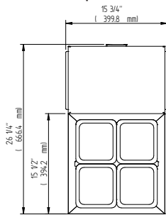
CPR-4 Top View
