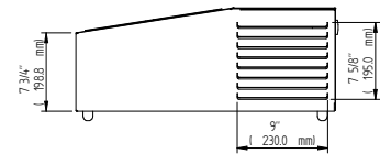
CPR-8 Side View
