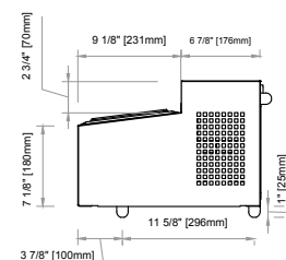
CPR-60-4 Side View
