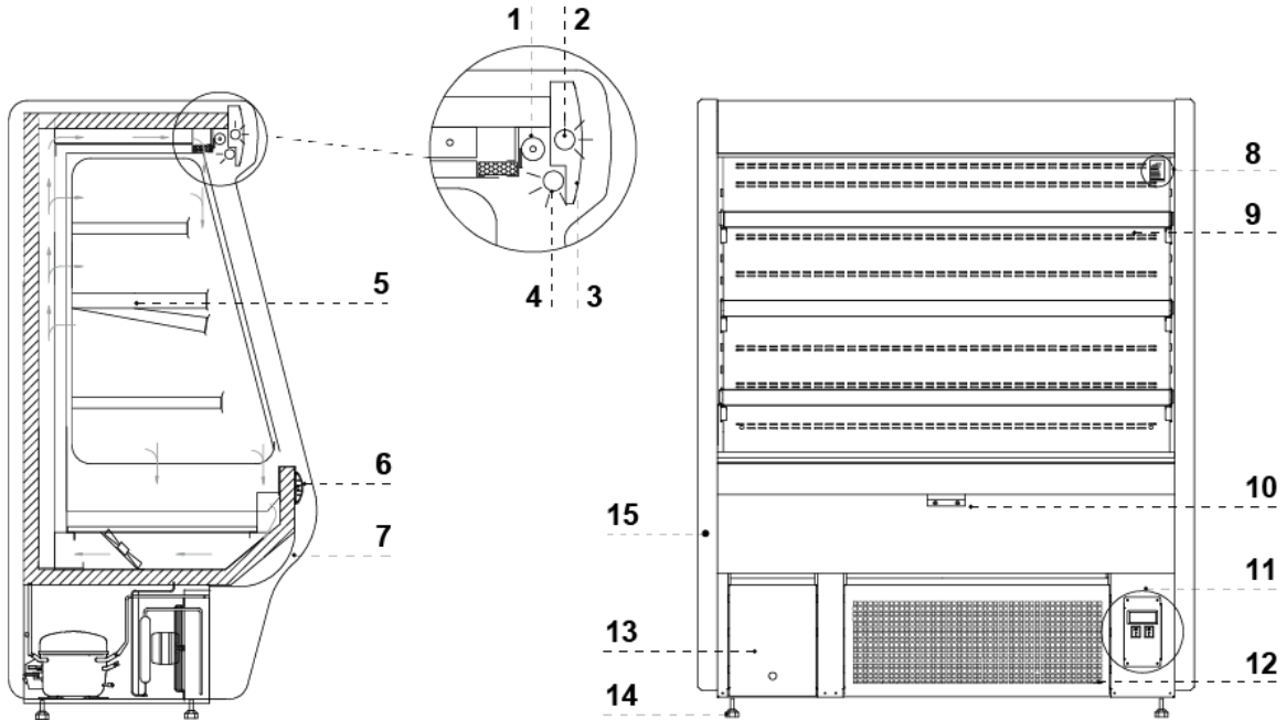
Figure 2 "6OM" overview
