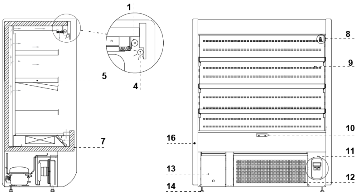
Figure 2 "6OM" overview
